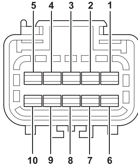
End View of Trailer Connector
