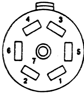
End View of Trailer Connector
