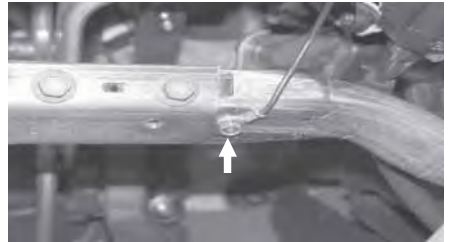
Center-Splice Procedure
